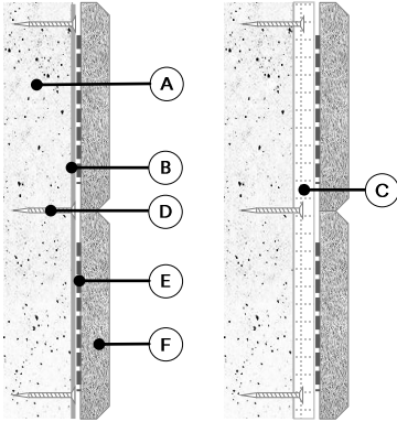
WM-A – Metal Sheets WM-B – Standard Cassettes
