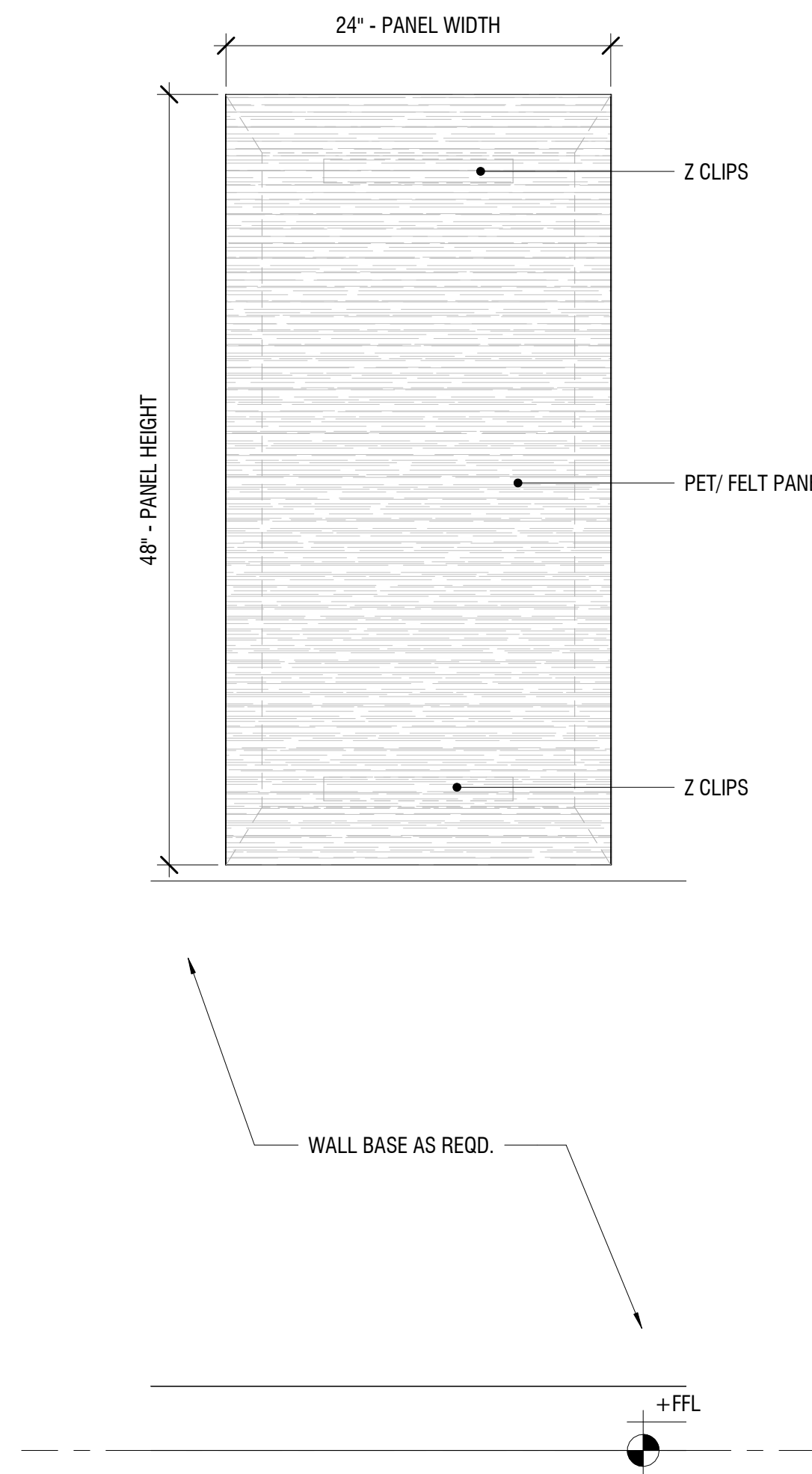
1 TOCKKY FWP - FELT WRAPPED PANEL 2x4' - ELEVATION 1 1/2" = 1'-0"
