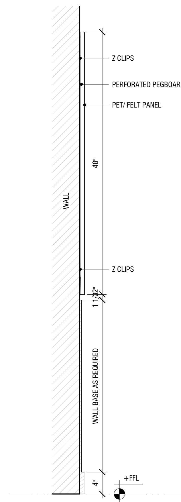
3 TOCKKY FWP - FELT WRAPPED PANEL 2x4' - TYP. SECTION 1 1/2" = 1'-0"
