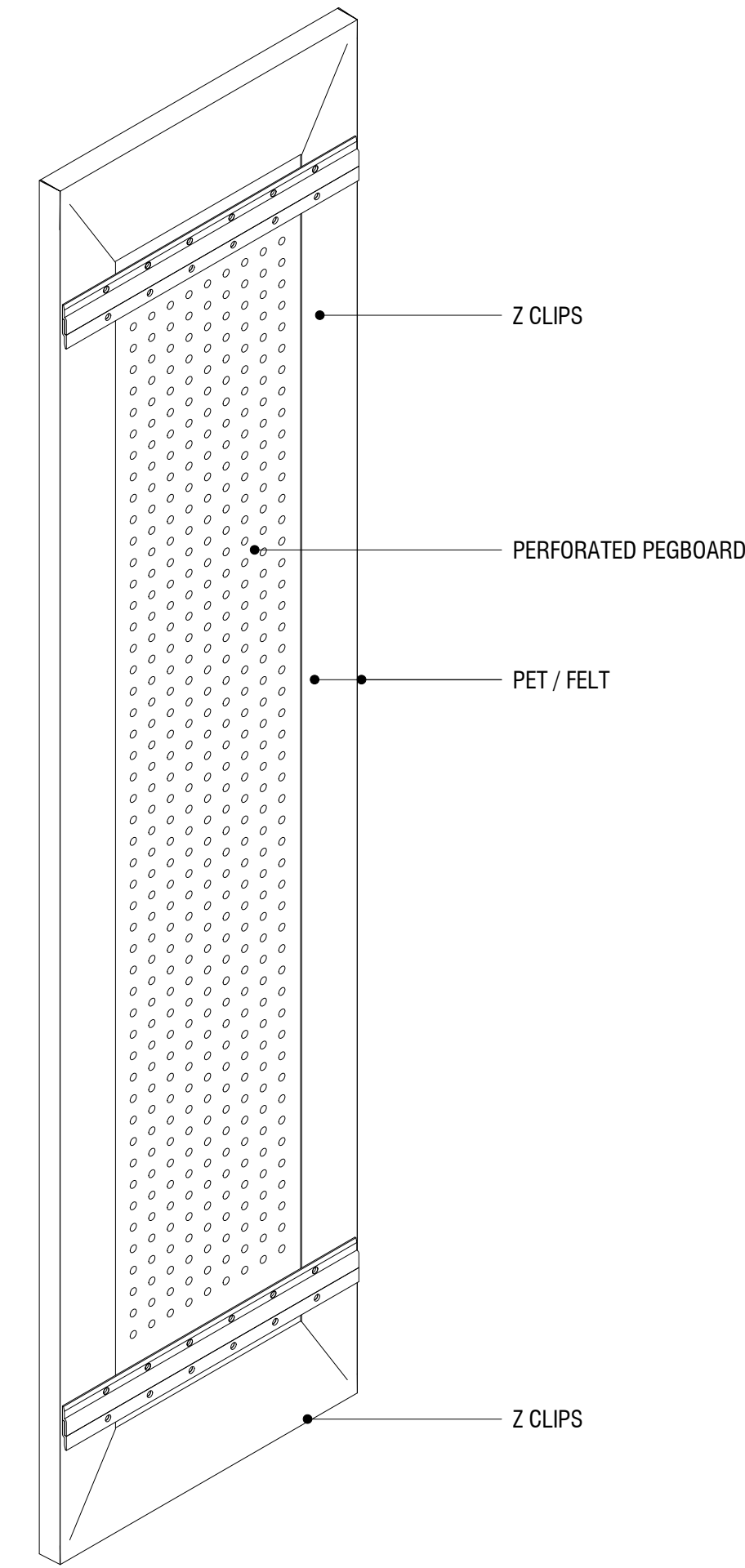
2 TOCKKY FWP - FELT WRAPPED PANEL 1x4' - AXONOMETRIC REAR VIEW
