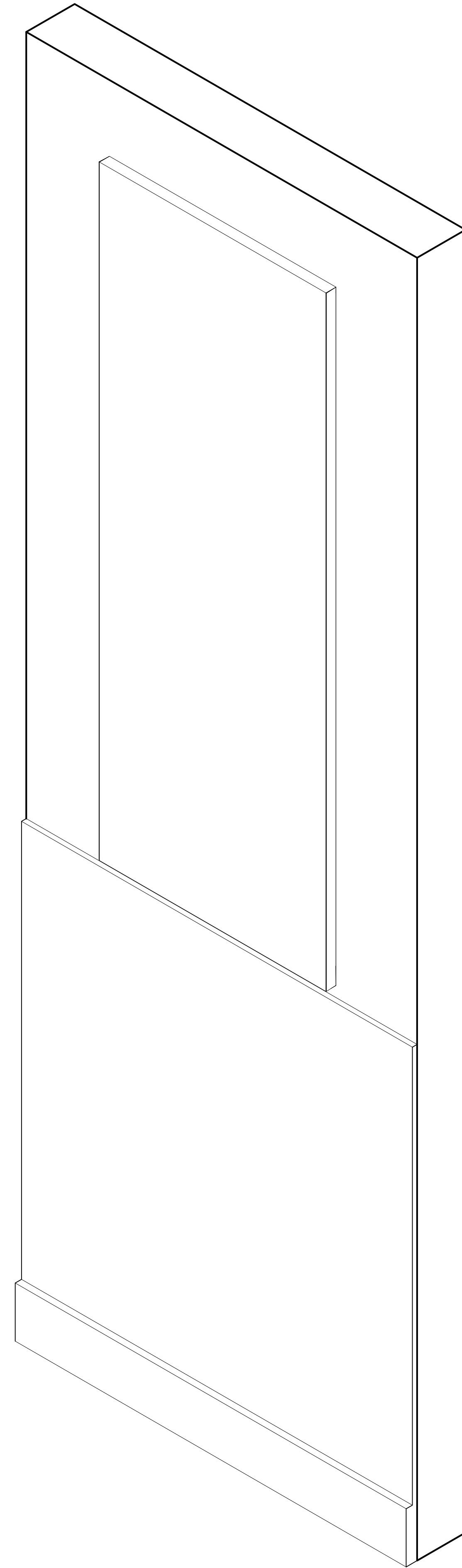
1 TOCKKY FWP - FELT WRAPPED PANEL 1 1/2'x4' - AXONOMETRIC FRONT VIEW
