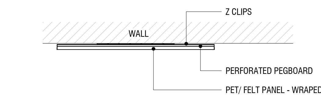
2 TOCKKY FWP - FELT WRAPPED PANEL 2x4' - PLAN VIEW 1 1/2" = 1'-0"
