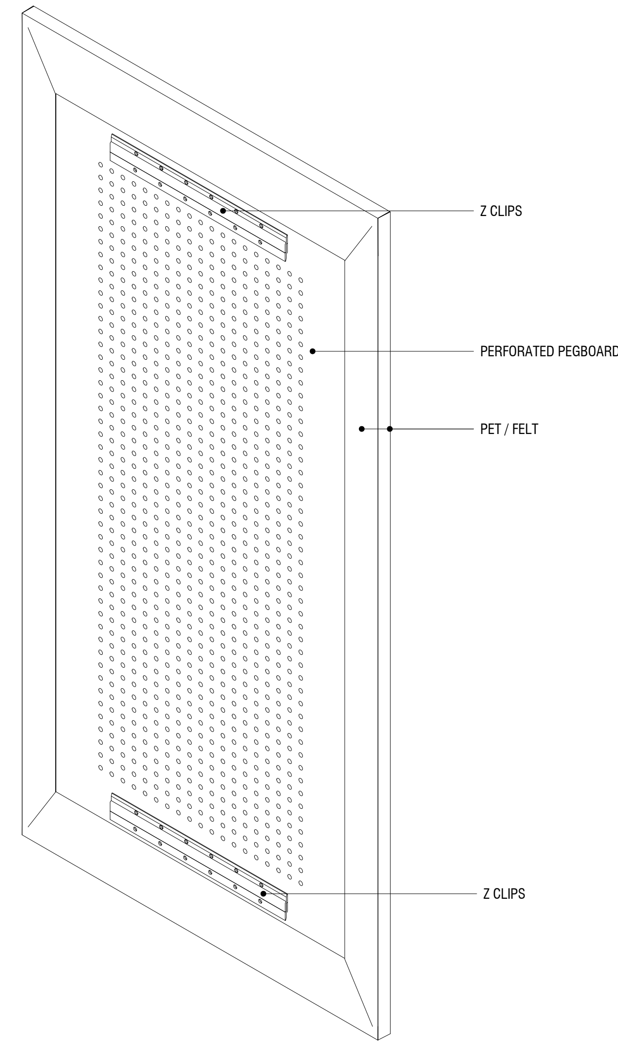
2 TOCKKY FWP - FELT WRAPPED PANEL 2x4' - AXONOMETRIC REAR VIEW
