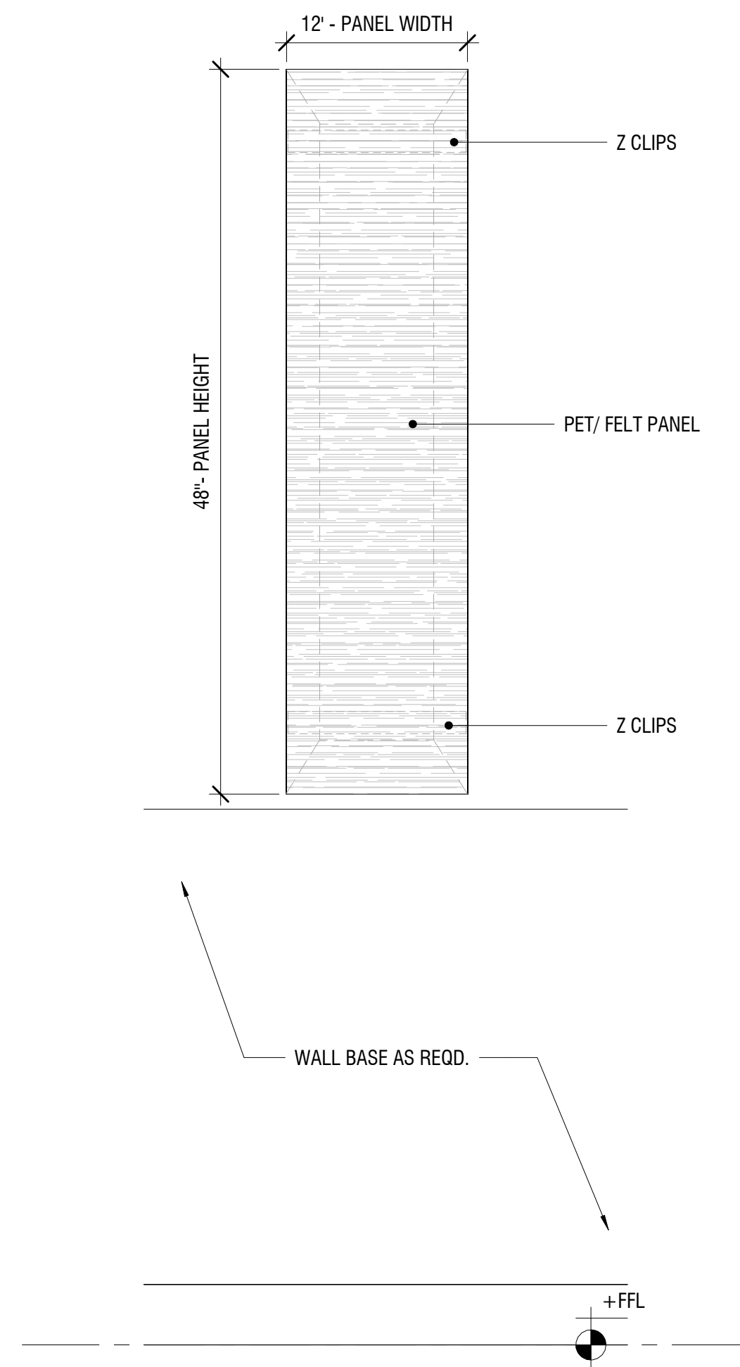
③ TOCKKY FWP - FELT WRAPPED PANEL 1'x4' - ELEVATION 1 1/2" = 1'-0"
