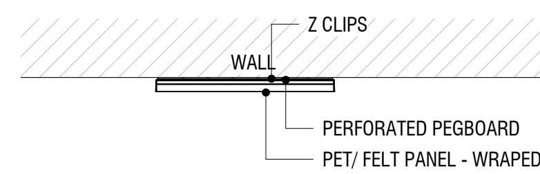
① TOCKKY FWP - FELT WRAPPED PANEL 1'x4' - PLAN VIEW 1 1/2" = 1'-0"
