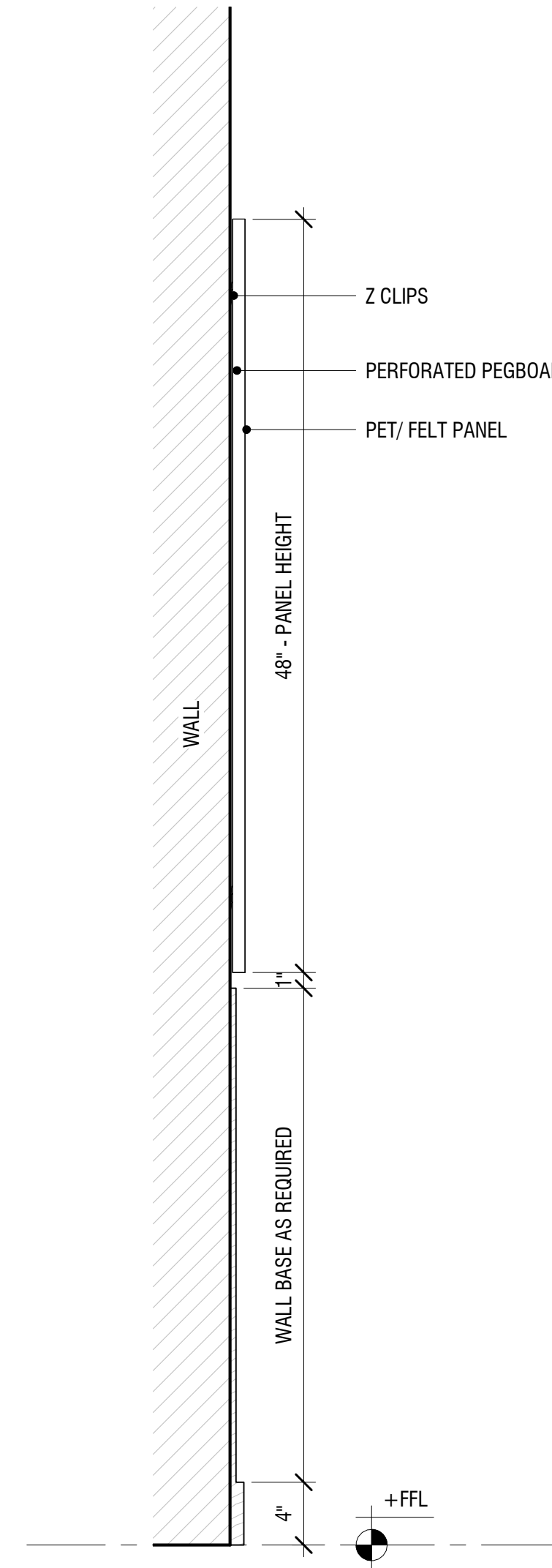
④ TOCKKY FWP - FELT WRAPPED PANEL 1'x4' - TYP. SECTION 1 1/2" = 1'-0"
