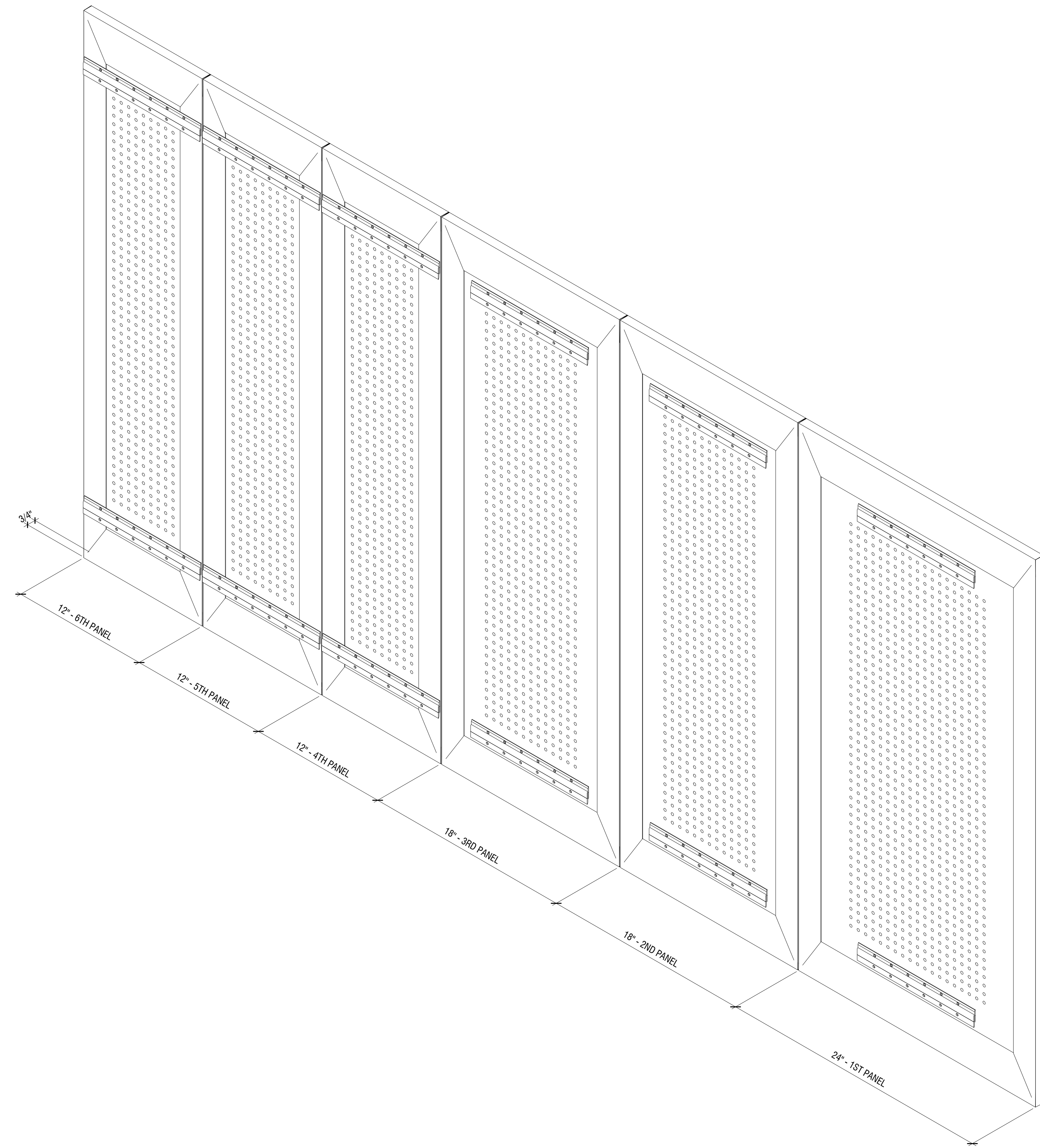
1 TOCKKY FWP - FELT WRAPPED PANELS ASSEMBLY 8'x4' - 3D AXON
