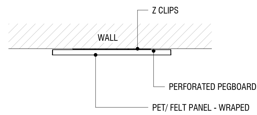
① TOCKKY FWP - FELT WRAPPED PANEL 1 1/2'x4' - PLAN VIEW 1 1/2" = 1'-0"
